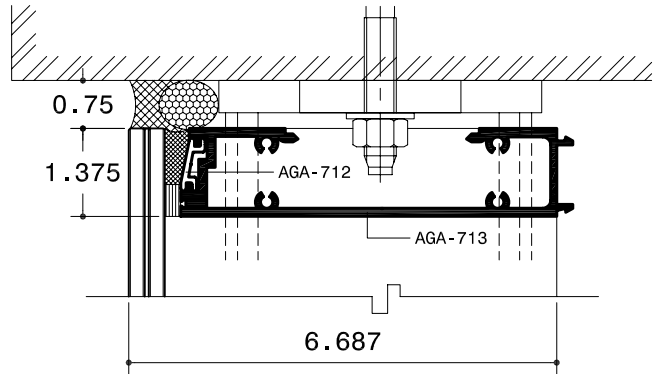
HEAD DETAIL
