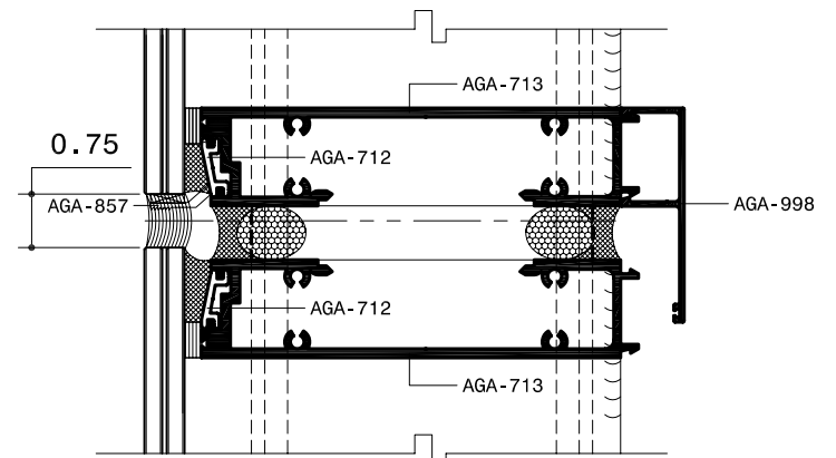
STACK JOINT DETAIL
