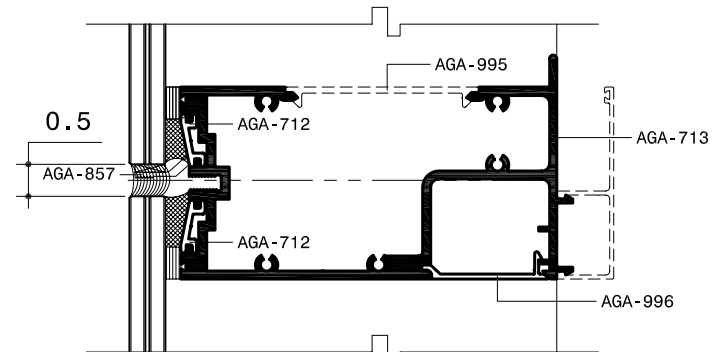
HORIZONTAL MULLION DETAIL
