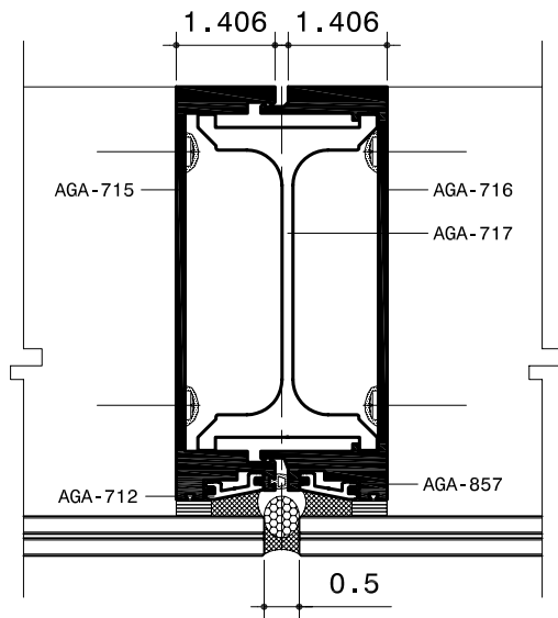
VERTICAL MULLION DETAIL
