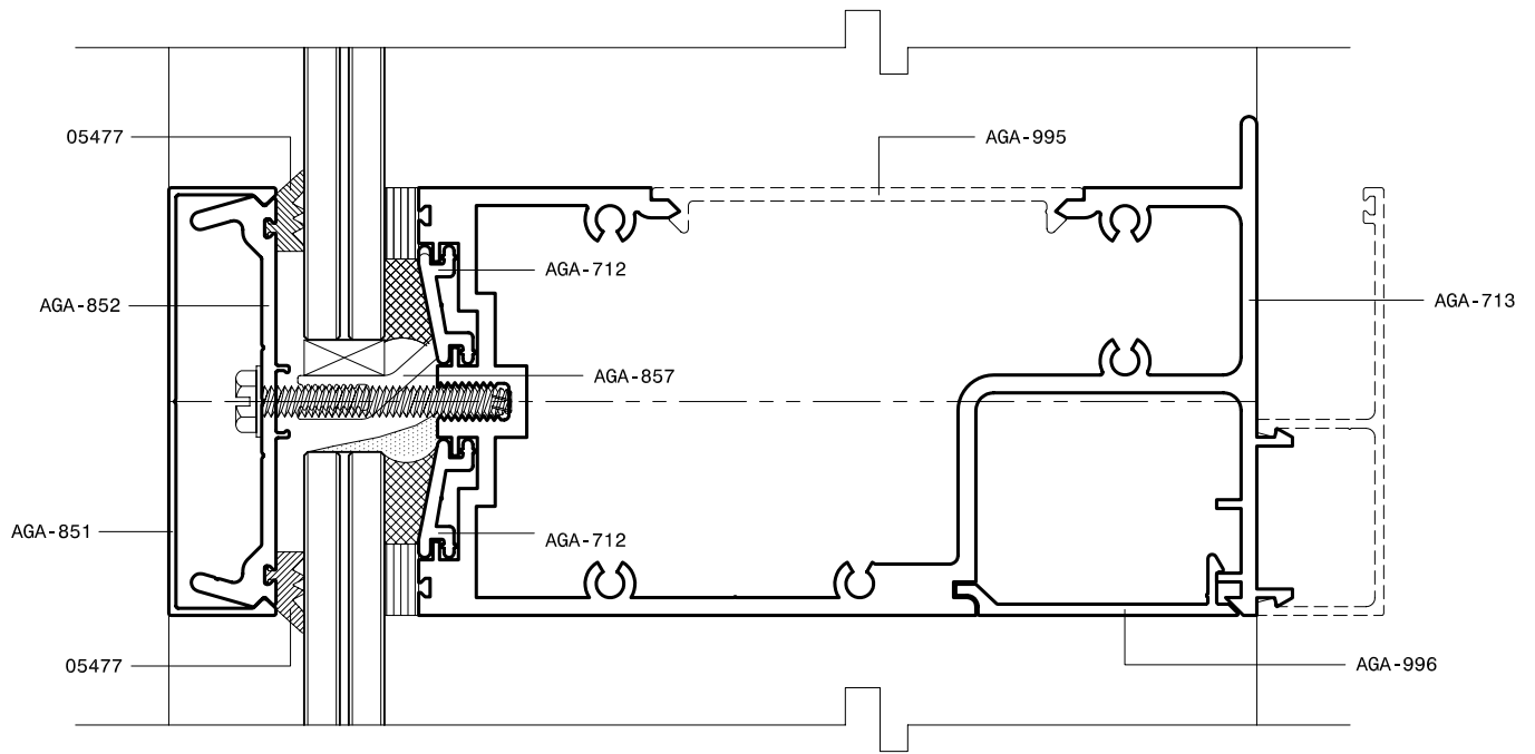
HORIZONTAL MULLION DETAIL WITH PRESSURE PLATE
