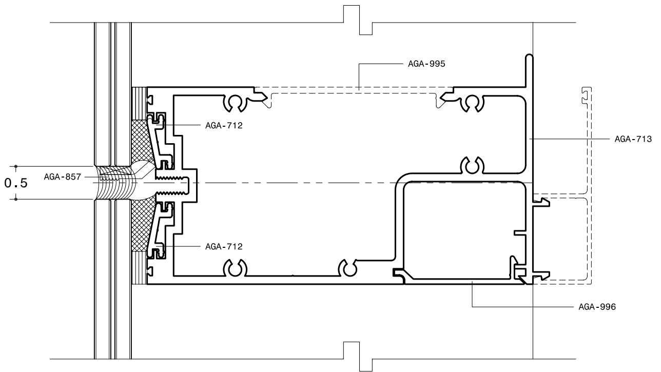
HORIZONTAL MULLION DETAIL STRUCTURAL GLAZED
