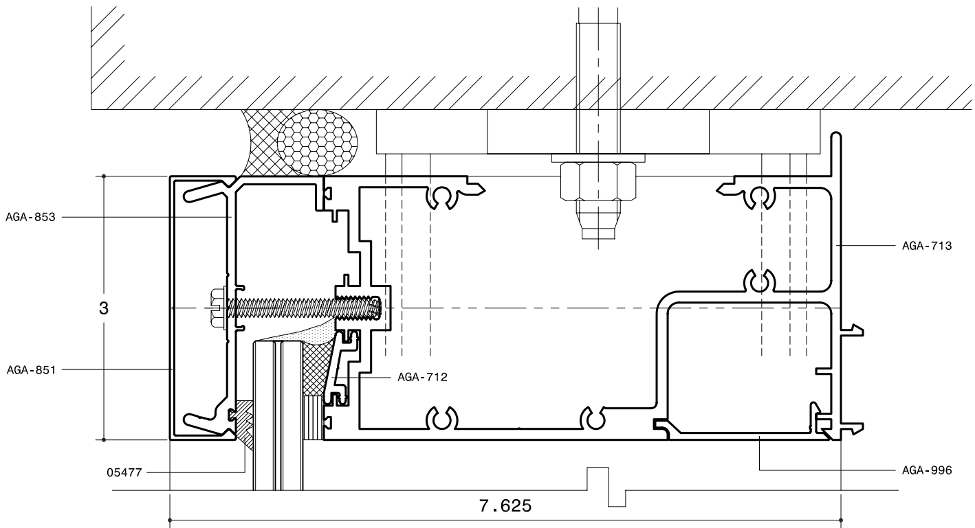
HEAD DETAIL WITH PRESSURE PLATE
