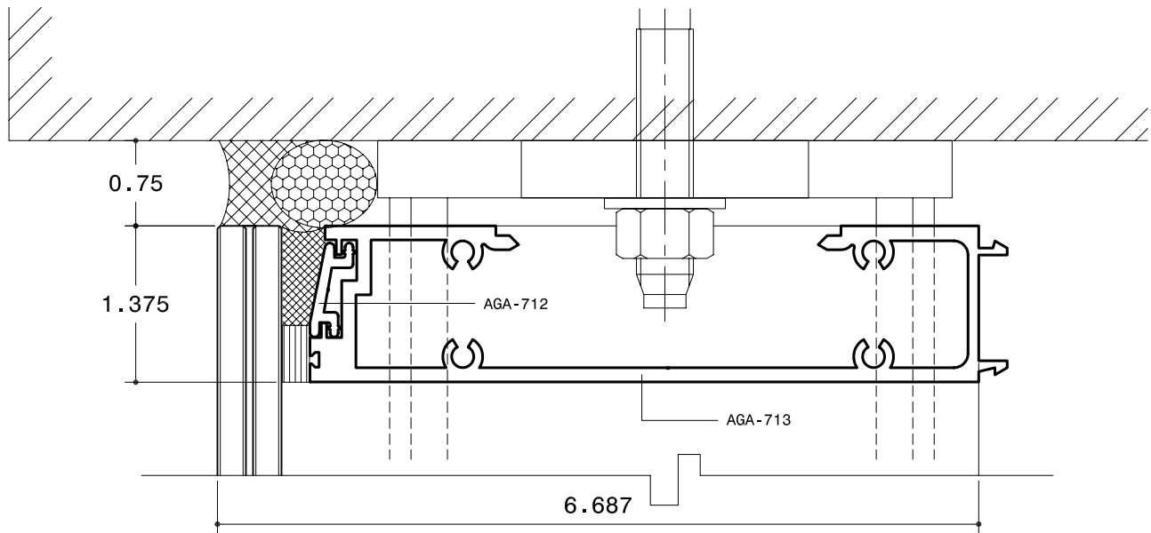
HEAD DETAIL WITH PRESSURE PLATE
