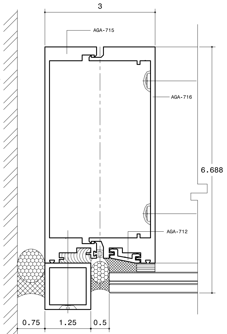
JAMB DETAIL STRUCTURAL GLAZED
