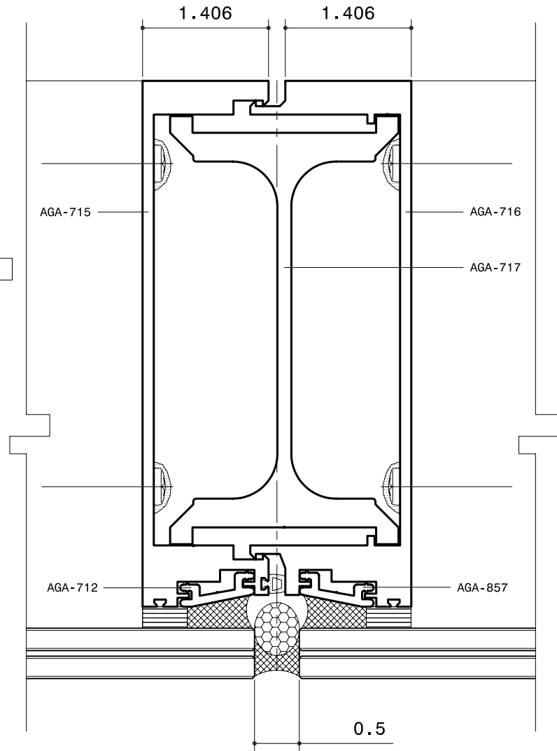
VERTICAL MULLION DETAIL STRUCTURAL GLAZED
