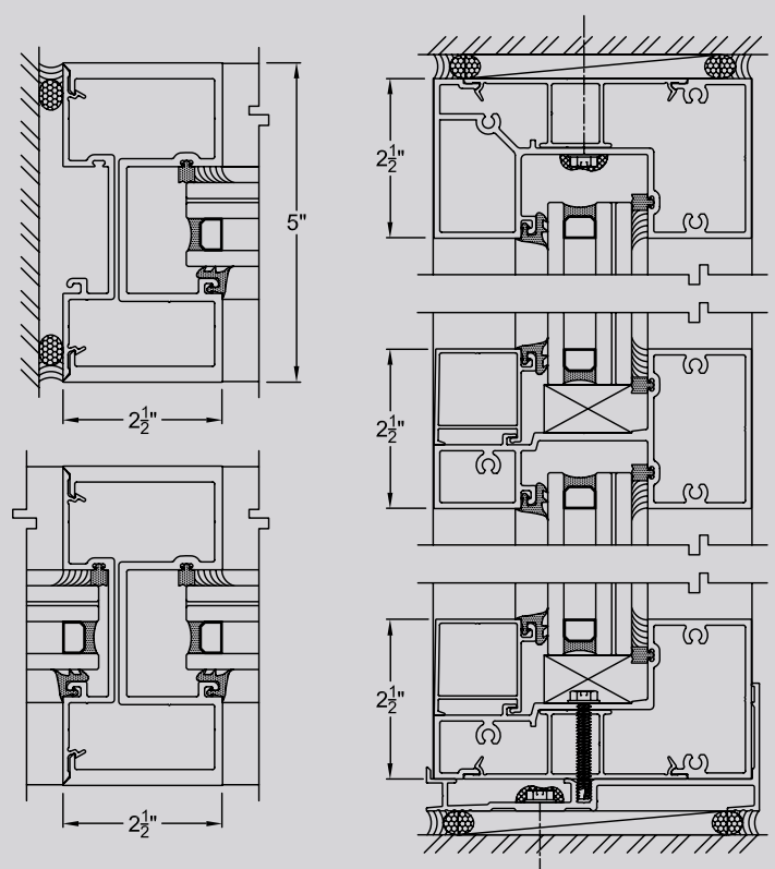
VERTICAL SECTIONS
