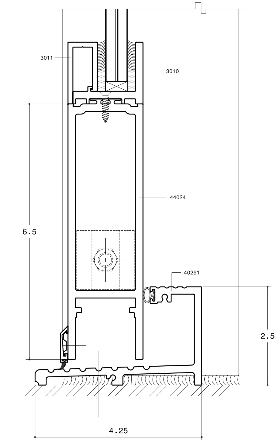
BOTTOM RAIL DETAIL
